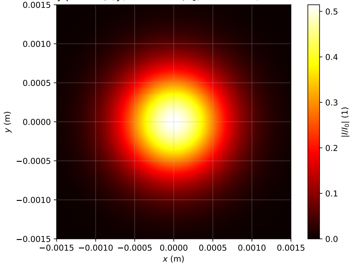
Intensity profile I(x, y, z = 2.548m)/I_0 , \text{Pin}=0.3\text{Pcr} , artificial time
